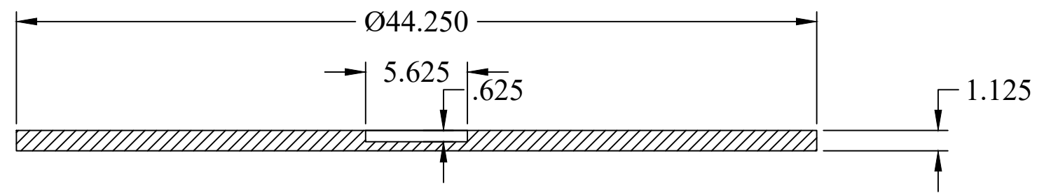
SECTION A-A COMPOSITE COVER
