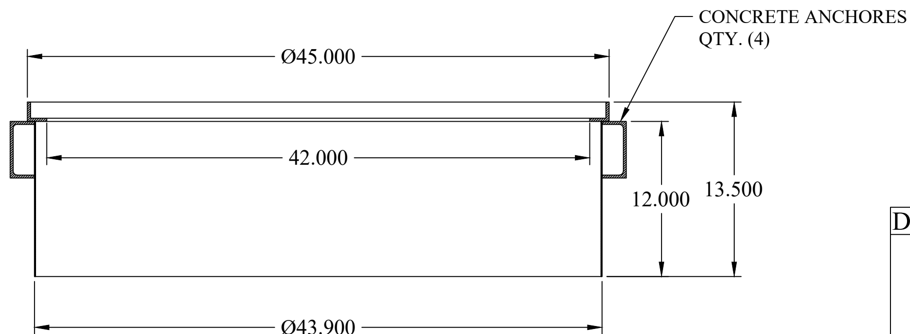
SECTION B-B (COVER NOT SHOWN)
