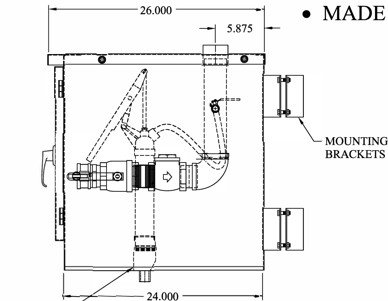
RIGHT SIDE RIGHT SIDE DRAIN FITTING
