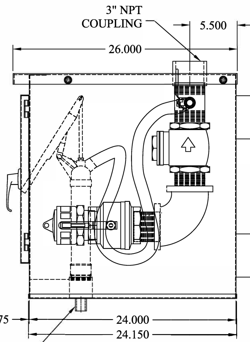
RIGHT SIDE
